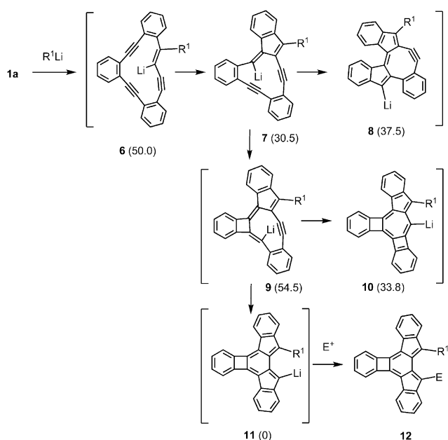
Scheme 1. A working hypothesis for tandem transannular cyclizations of 1a . Energies ( \text{kcal mol}^{-1} ), relative to 11 , were calculated by a DFT ((R)B3LYP/6-31G*) method and are shown within parentheses.
